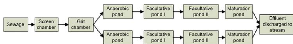
Figure 17.6 Schematic flow chart of WSP Agra.
