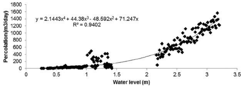
Figure 7.5 Relationship between the water level and the percolation rate in the tank.
