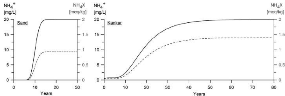
Figure 4.6 Results of adsorption modelling. Solid black line: Ammonium concentration in the water in mg/L (shown on the primary y-axis), dashed grey line: Ammonium concentrations on the exchanger in meq/kg sediment (shown on the secondary y-axis). The amount of ammonium sorbed on the sediment depends on the number of exchange sites available, on the solute composition and on the selectivity coefficients, which are sediment-dependent. It can be clearly seen that more ammonium can be adsorbed on the kankar material than on the sand.
