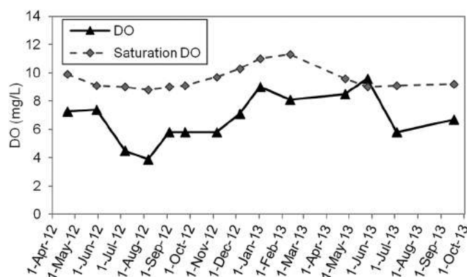
Figure 3.7 Dissolved oxygen (DO) concentration of the lake at its surface and its saturation concentration at the water temperature as a function of time.
