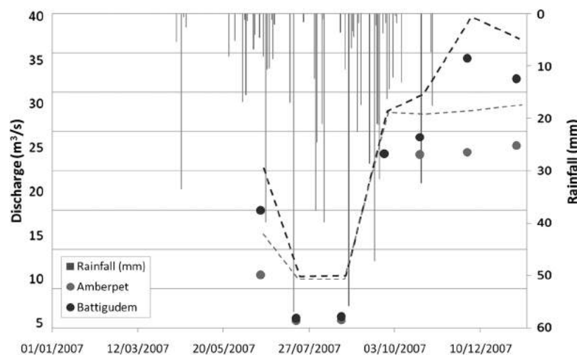
Figure 11.4 Discharge rate ( \text{m}^3/\text{s} ) measurements of the Musi River at Amberpet and Battigudem from May 2007 to January 2008 and daily rainfall (mm) in Hyderabad from January 2007 to January 2008.
