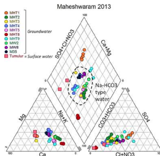
Figure 7.9 Piper diagram for groundwater (10 wells) and Tummulur tank surface water for the 2013–2014 campaign.
